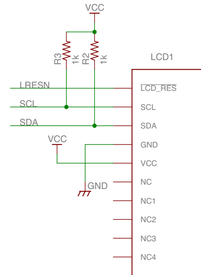
I2C LCD 3.3V Strawberry-LINUX
